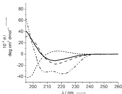
Figure 1. CD spectrum of an ESI solution of Ac-A 15 K (76 \mu M) in 50:50 v/v methanol/water with 1% acetic acid (—) in comparison with standard CD spectra of pure \alpha -helix (—), \beta -sheet (---) and random-coil (----) conformations.
